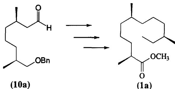
Scheme 5. Synthesis of methyl (2 S ,6 S ,10 S )-2,6,10-trimethyldodecanoate ( 1a ).
