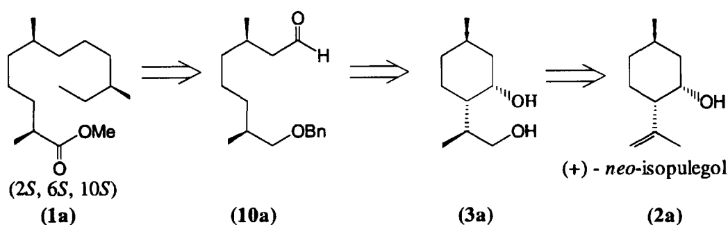
Scheme 1. Retrosynthetic analysis.
